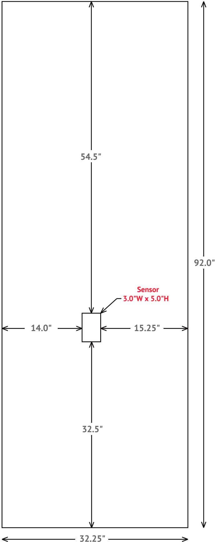
Light Box L1-B02 Panel "A" Detail
