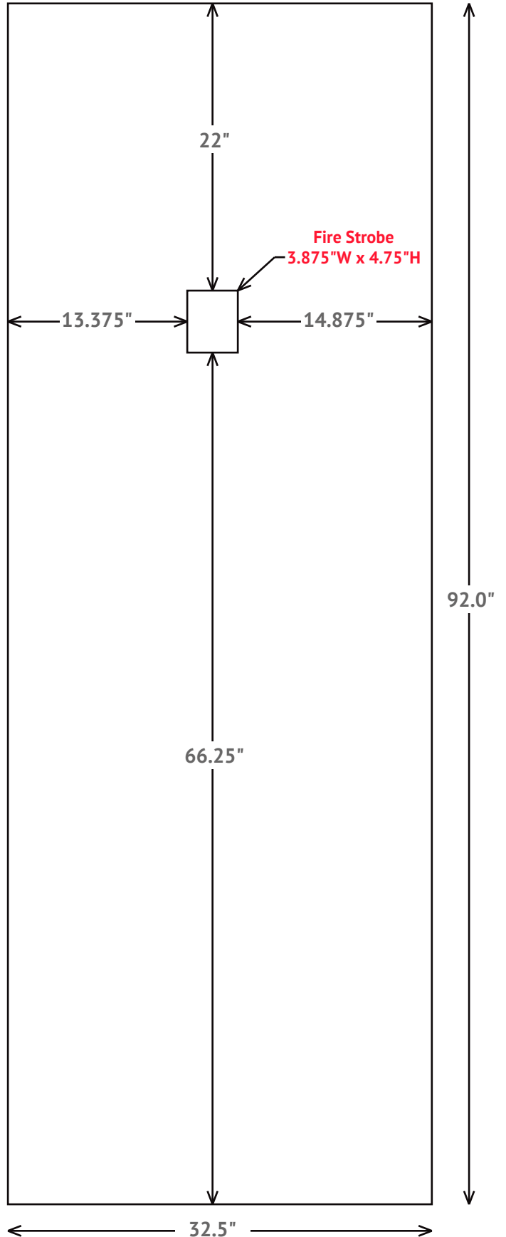
Light Box L1-B02 Panel "C" Detail
