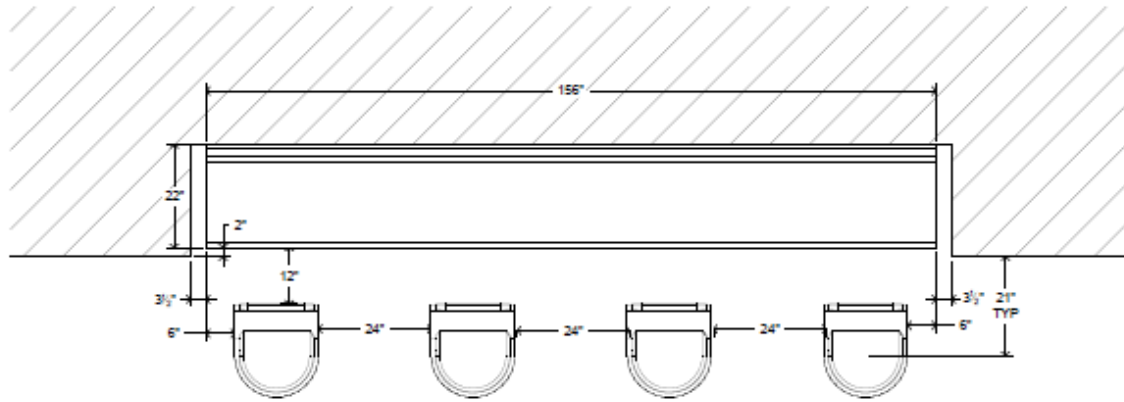
PLAN VIEW SCALE: 3/4" = 1'
