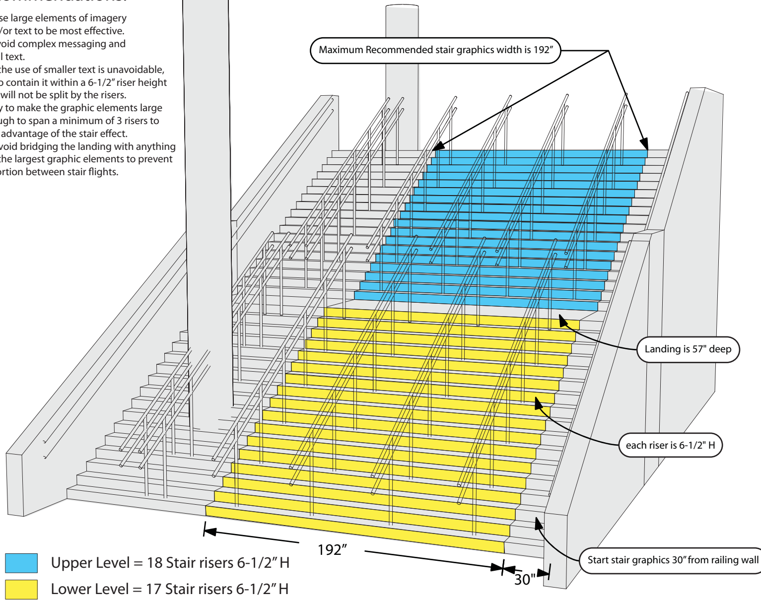
PERSPECTIVE VIEW
