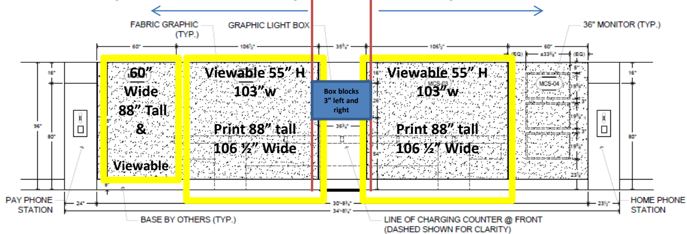
ELEVATION - MAIN CHARGING STATION (BACK WALL)
