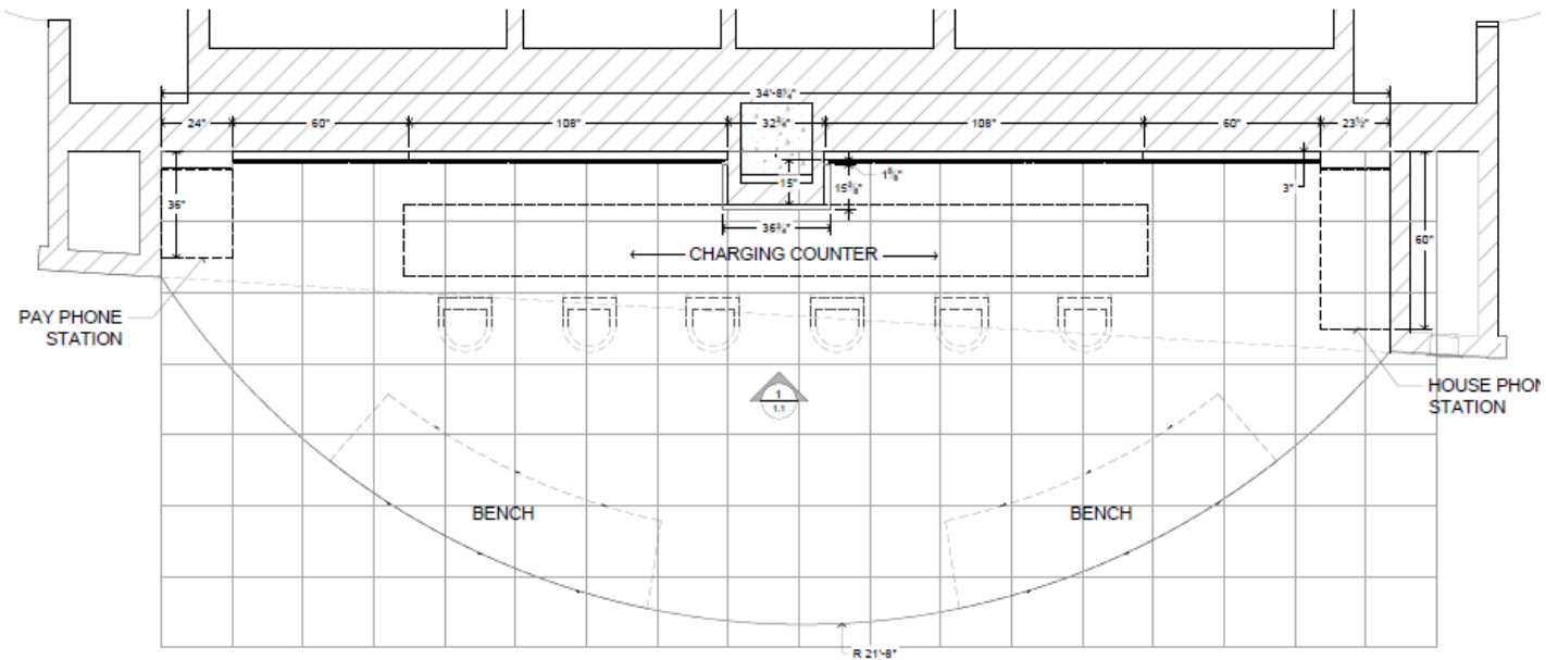
PLAN VIEW - MAIN CHARGING STATION (BACK WALL)
