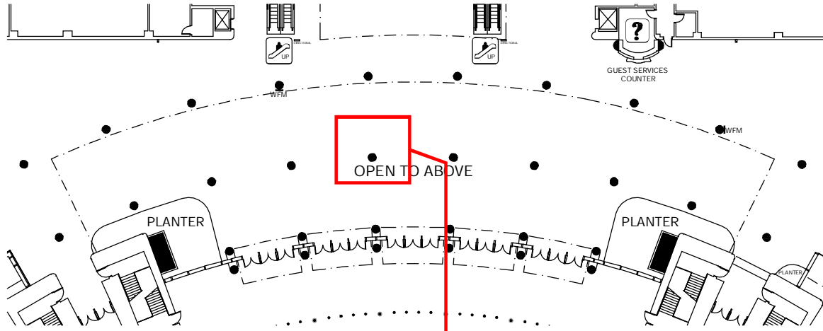
WEST BUILDING LEVEL TWO - WEST C LOBBY - CENTER COLUMNS 20 TYPICAL AT MAIN ENTRANCE
