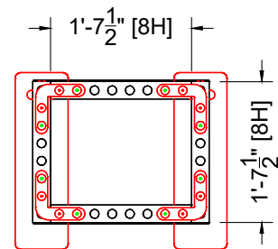
PLAN VIEW Scale: 1/2" = 1'-0"
