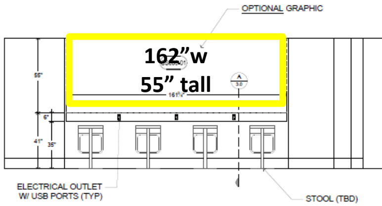
ELEVATION A - 600's CHARGING STATION SCALE: 1/2" = 1'
