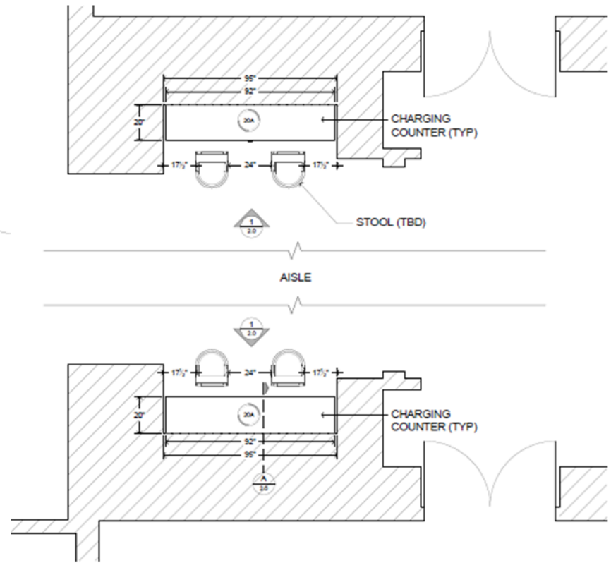
PLAN VIEW - 700's CHARGING STATIONS SCALE: 1/2" = 1'
