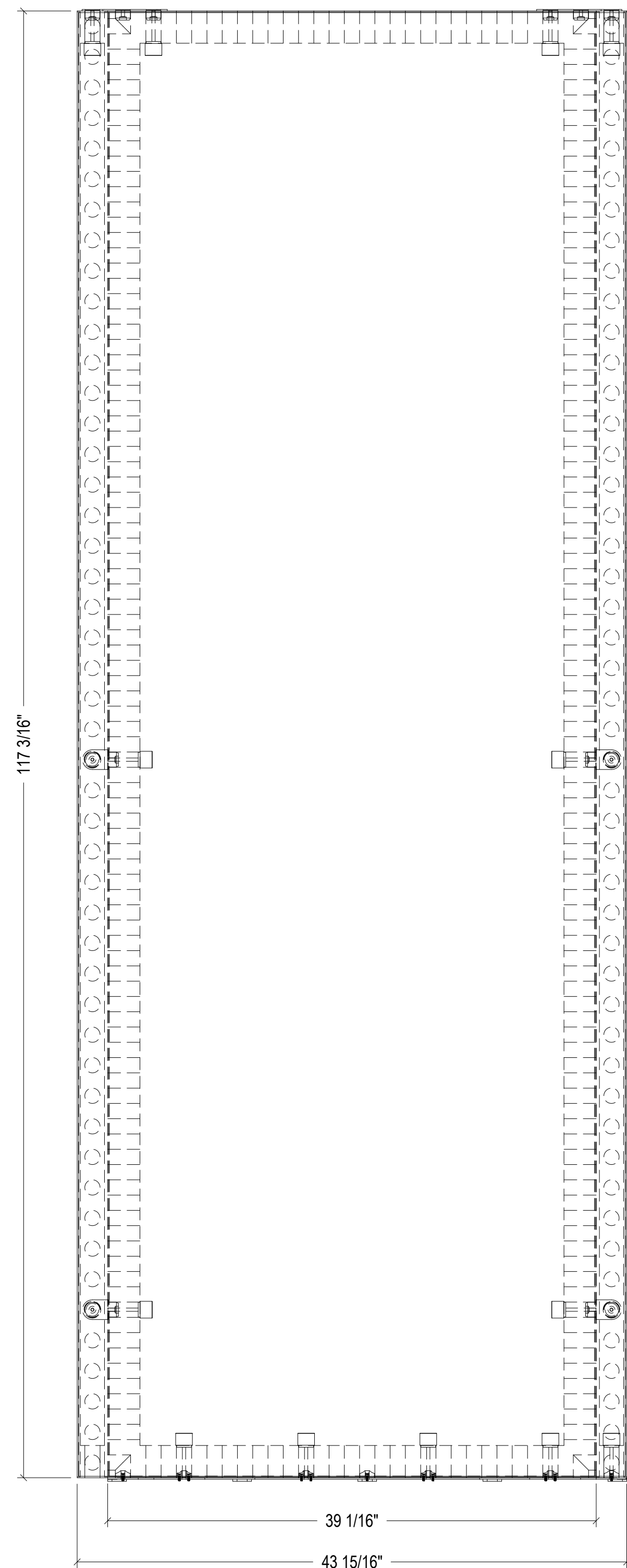
2 FLEX BY FREEMAN - 48 HOLE OUTDOOR TOWER - SIDE ELEVATION D-1.1 SCALE: 1-1/2"=1'-0"
