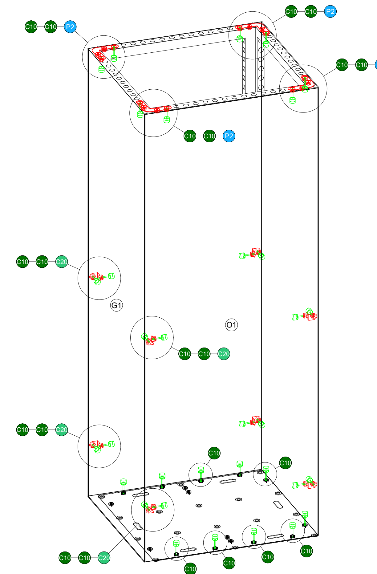
4 FLEX BY FREEMAN - 48 HOLE OUTDOOR TOWER - ISOMETRIC VIEW D-1.1 SCALE: NTS
