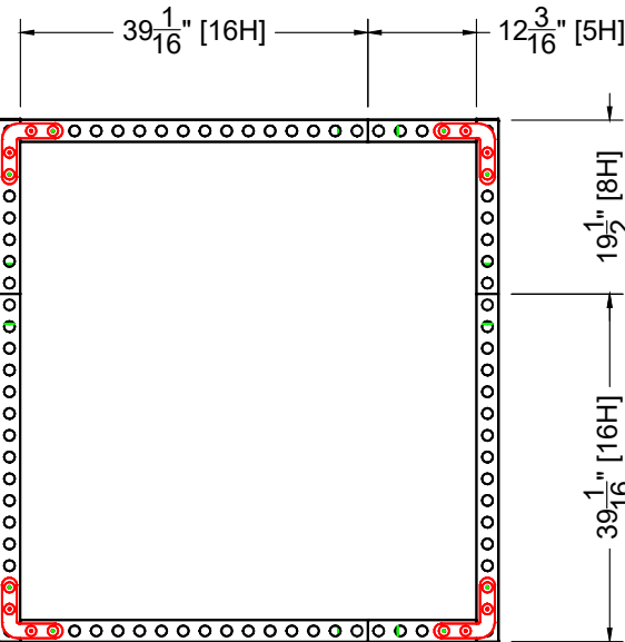
PLAN VIEW Scale: 1/2" = 1'-0"
