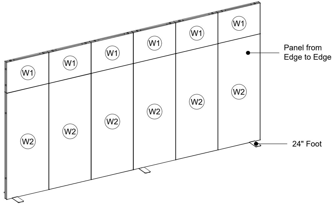
3D VIEW - FRONT
