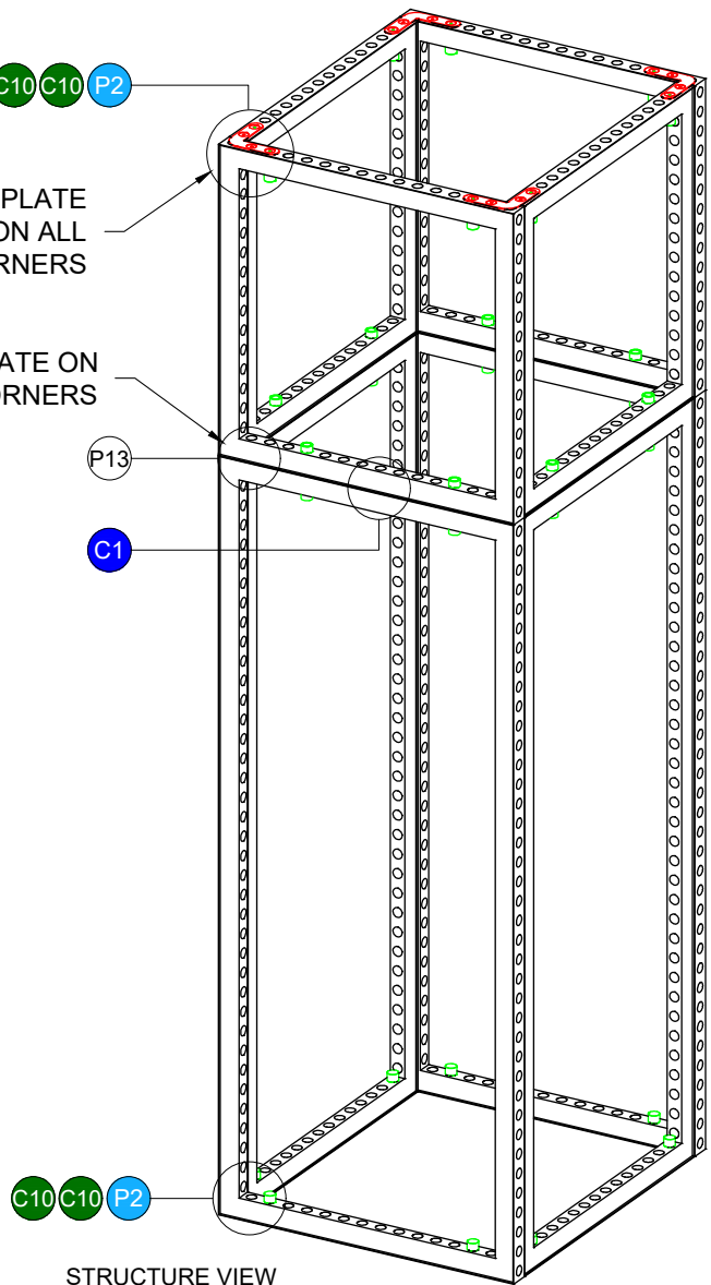
STRUCTURE VIEW
