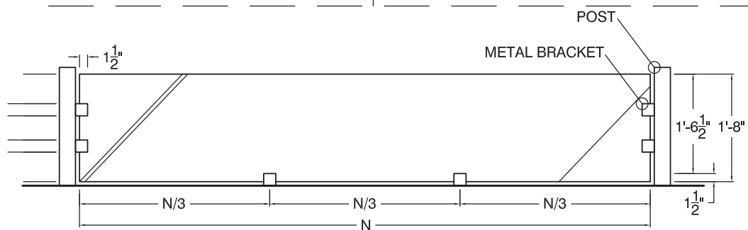
DETAIL OF INDIVIDUAL GLASS PANEL
