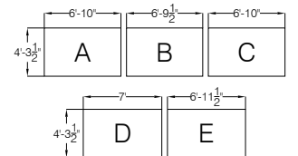
WINDOW DIMENSIONS - C-205 ELEVATION VIEW
