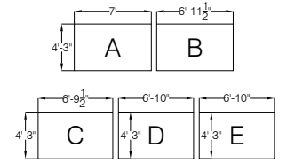
WINDOW DIMENSIONS - C-206 ELEVATION VIEW
