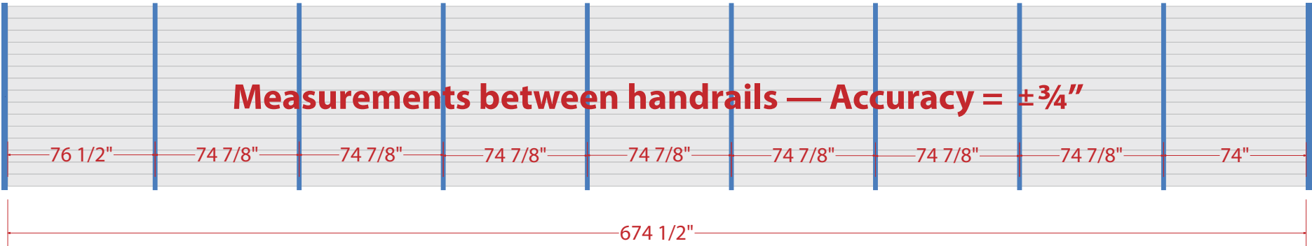
Center Staircase — Total: 15 risers 56'-2½" w x 6¼" h
