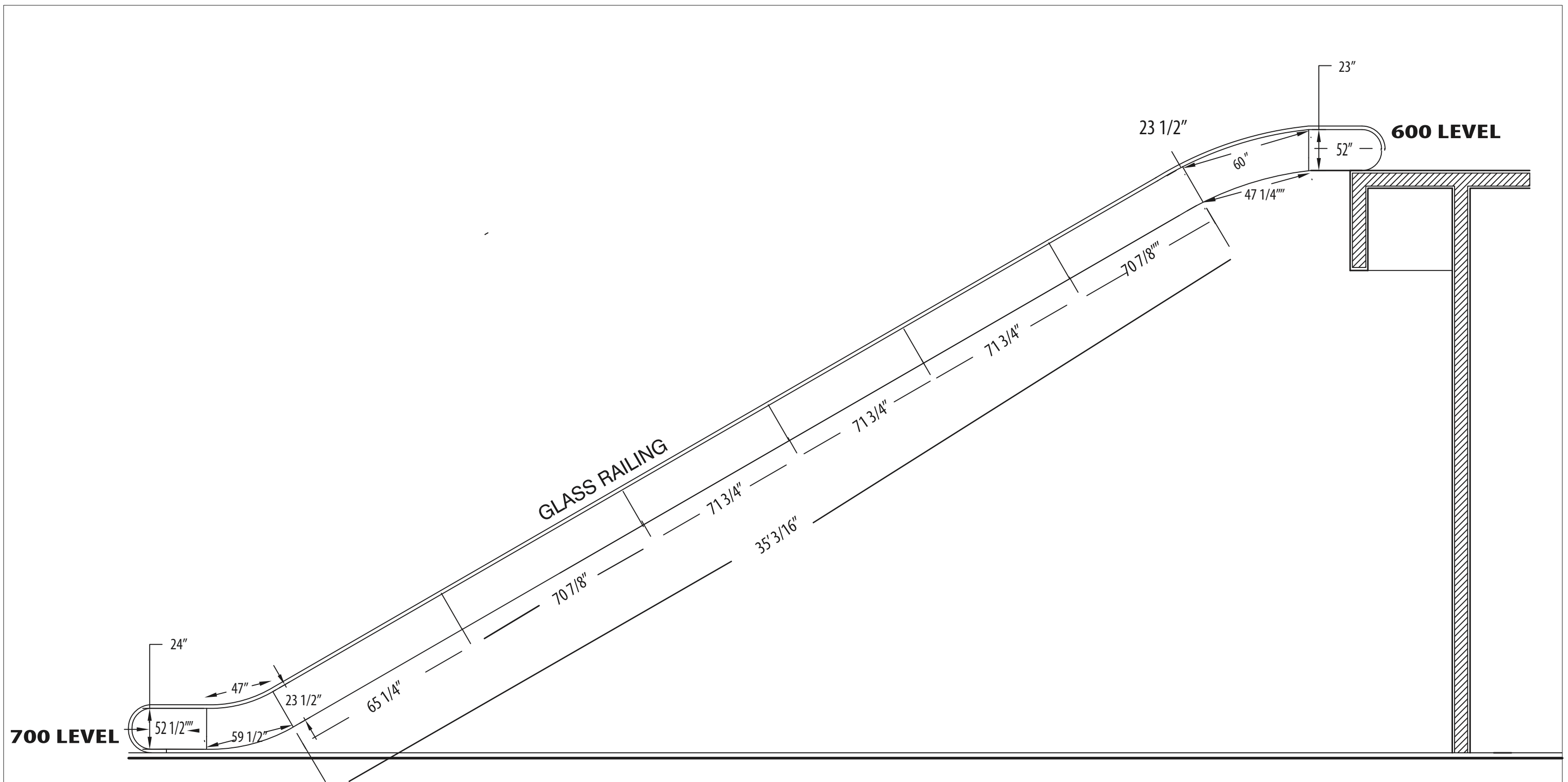
SOUTH - 600 LEVEL - 700 LEVEL - Outside escalator
