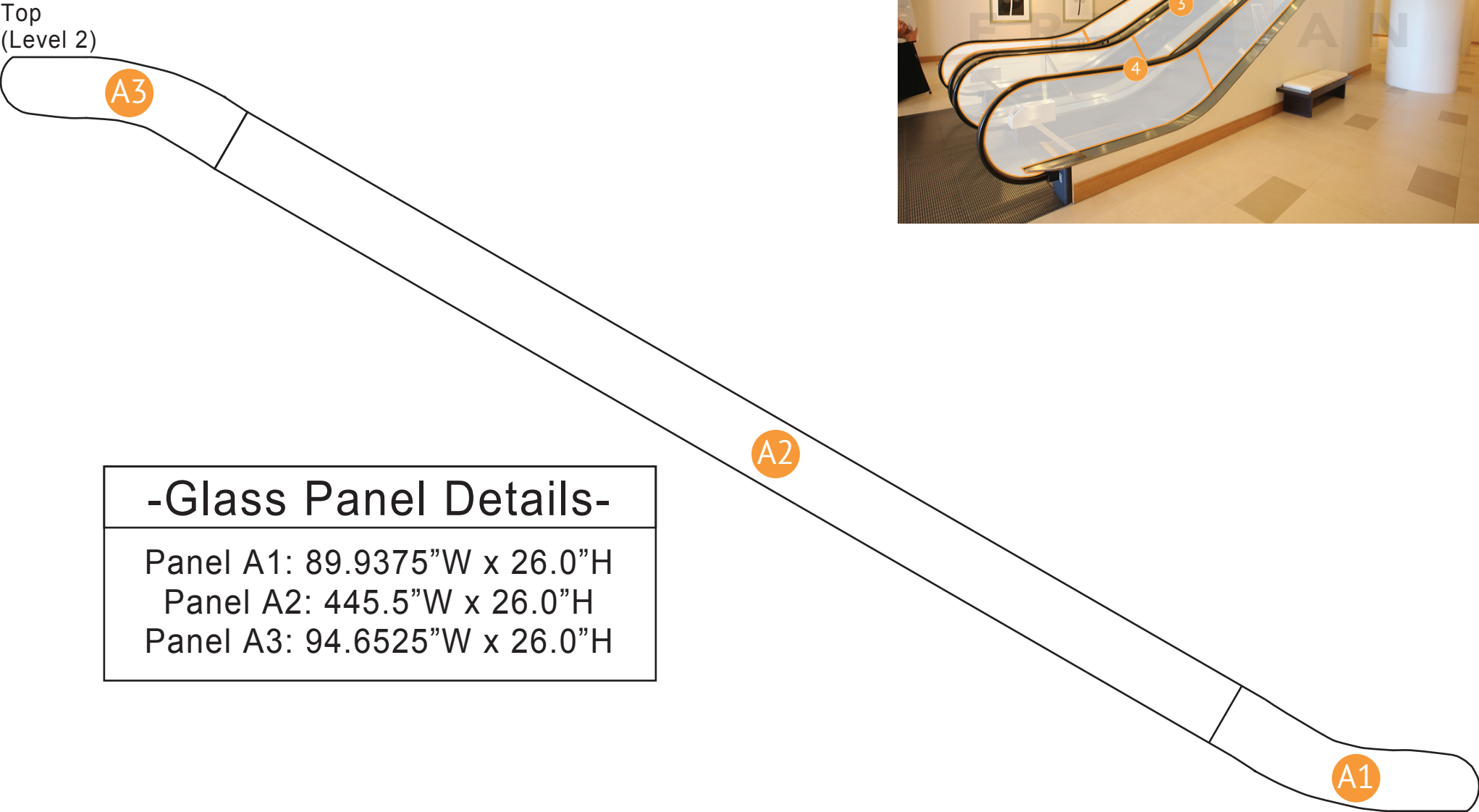
PlanTour Escalator Detail Drawing Not To Scale
