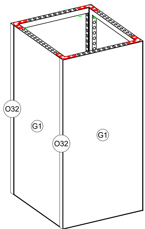
BACK VIEW
