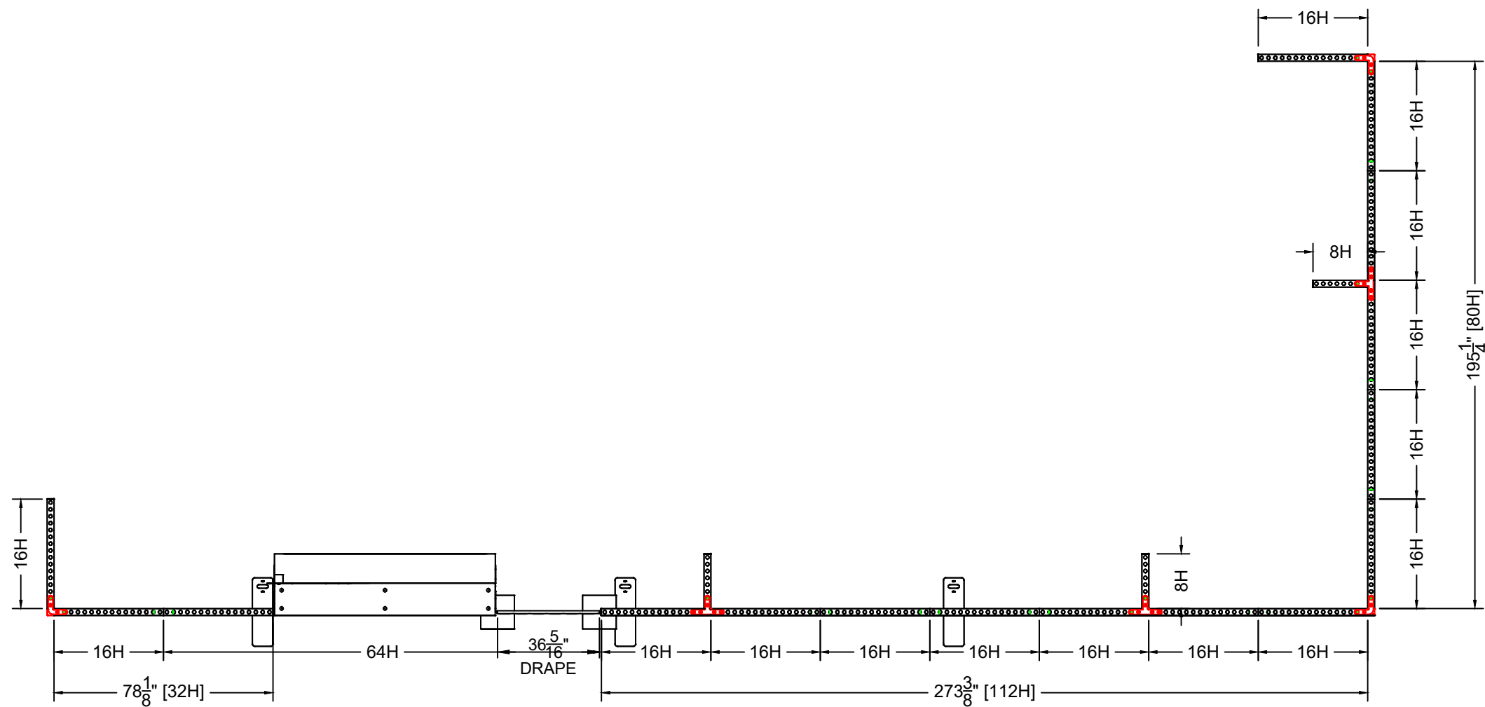
PLAN VIEW
