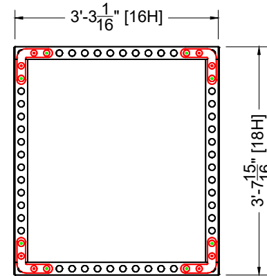
PLAN VIEW Scale: 1/2" = 1'-0"
