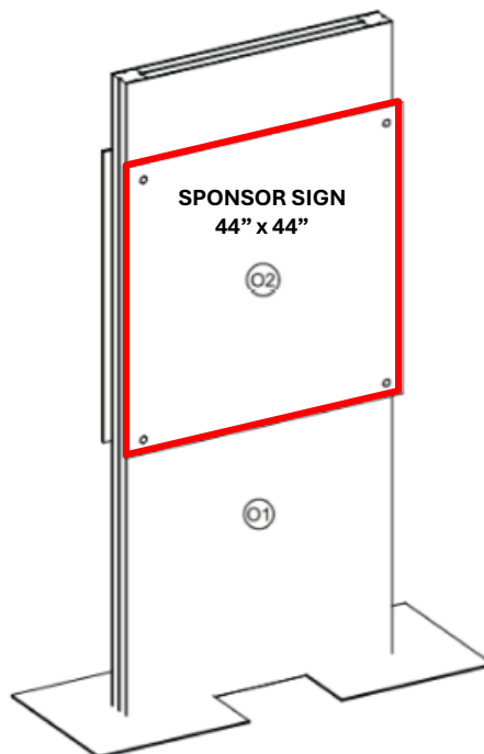
.375" Eyeholes for bumpouts Placement of the eyeholes are 2" down and 2" in from the sides
