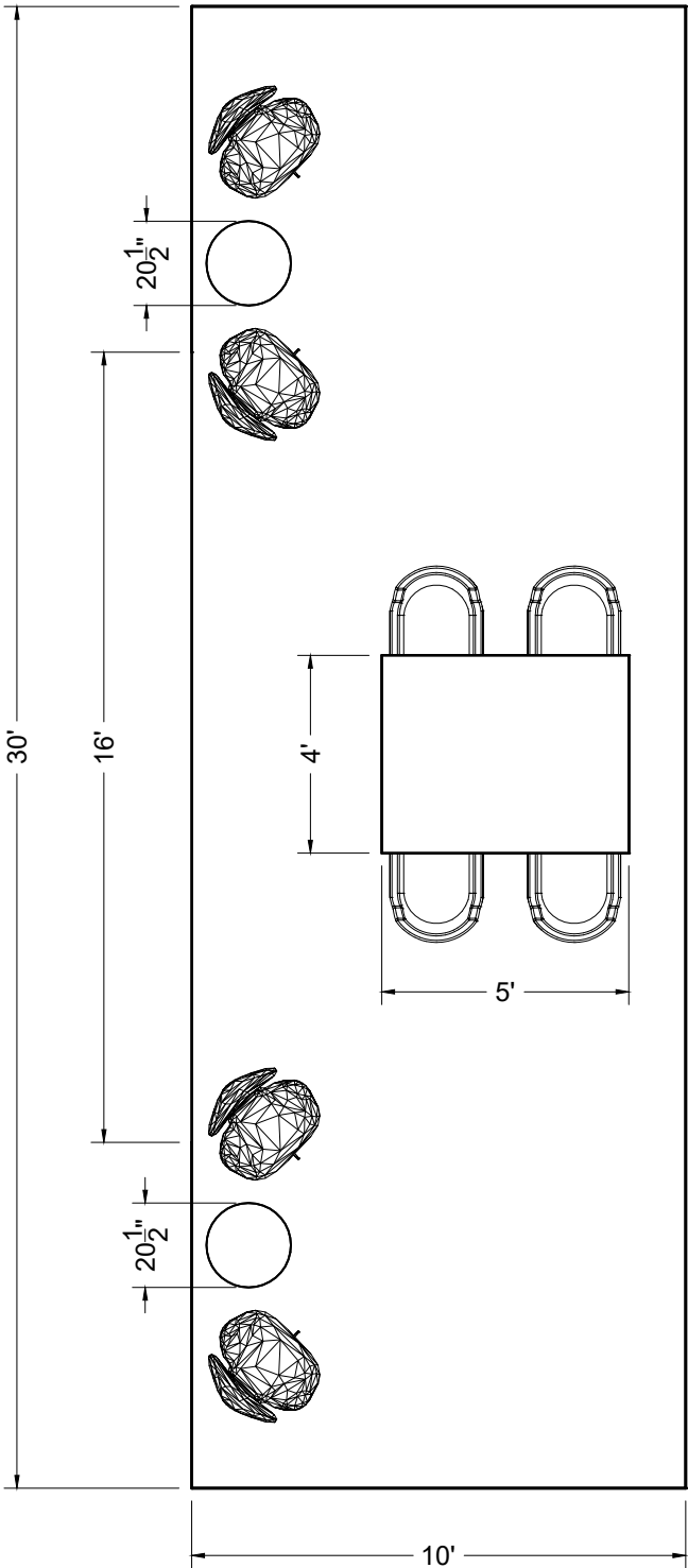
PLAN VIEW
