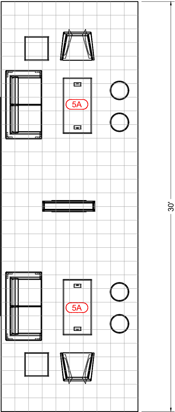
ELECTRICAL LAYOUT GRID SPACING = 1' X 1'
