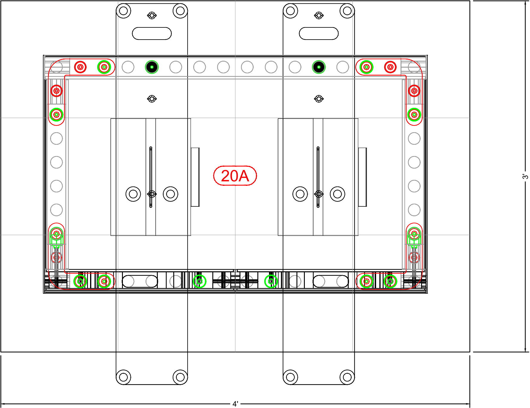
ELECTRICAL LAYOUT GRID SPACING = 1' X 1'
