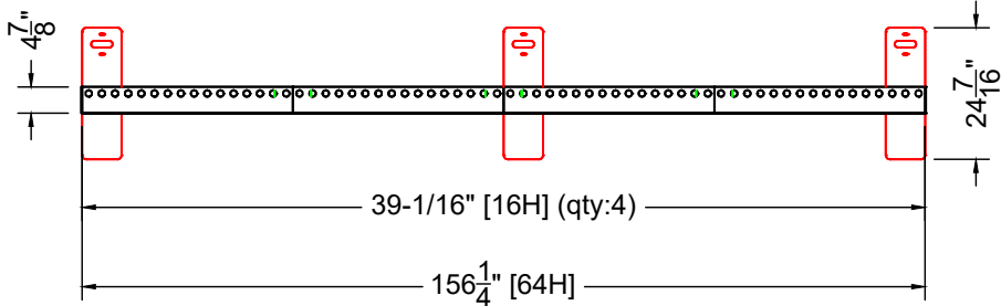
PLAN VIEW
