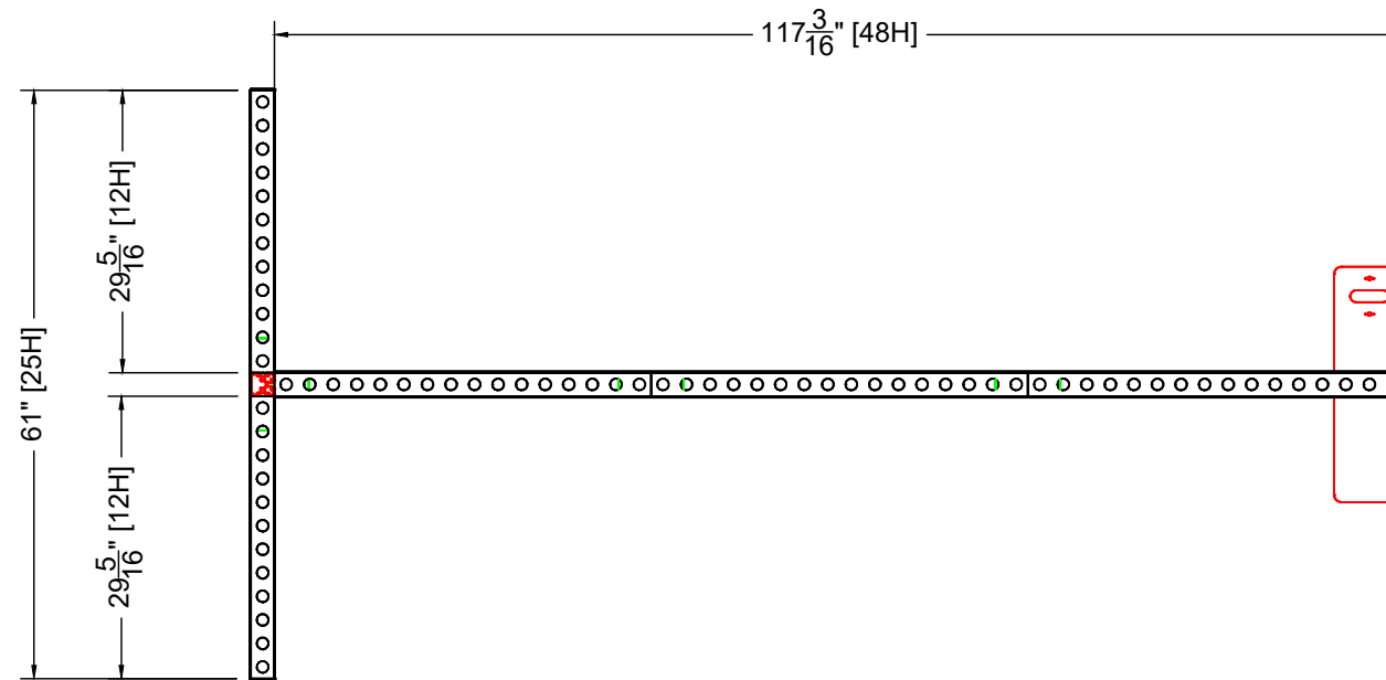
PLAN VIEW
