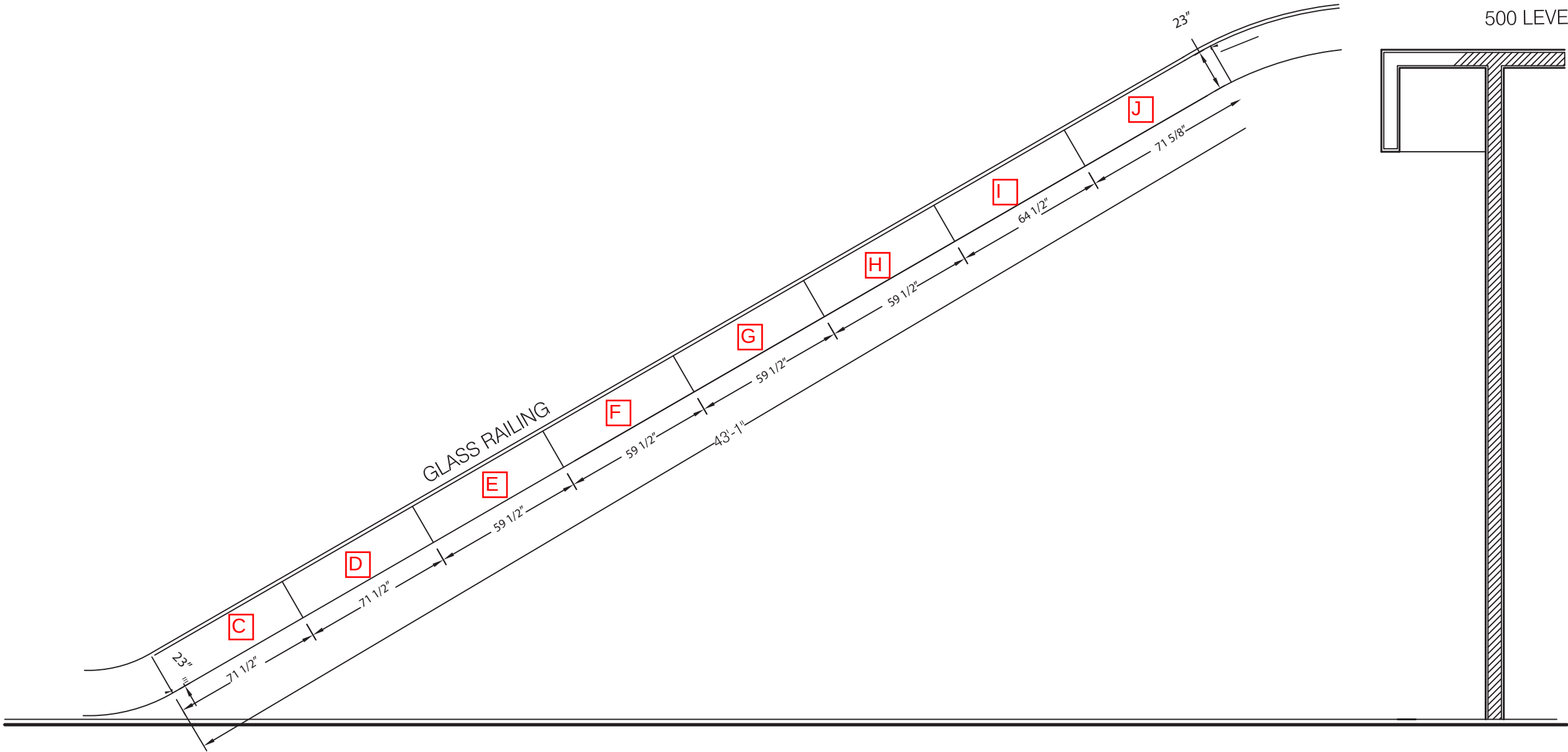
OUTER LEFT AND RIGHT ESCALATOR - SECTION
