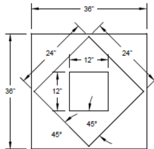
PLAN VIEW
