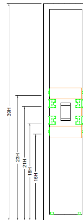
FRONT ELEVATION Scale: 3/4" = 1'-0"
