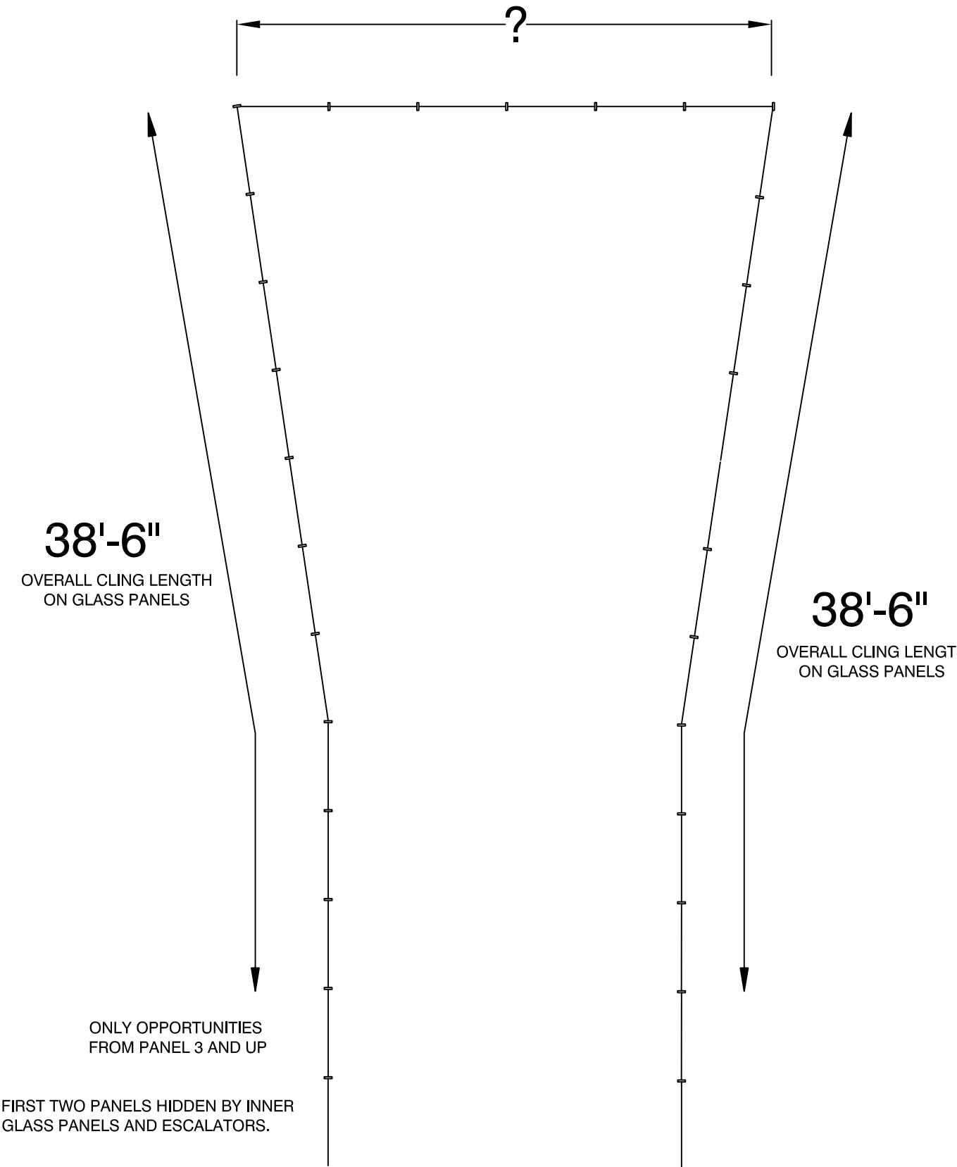
OVERALL DIMENSIONS
