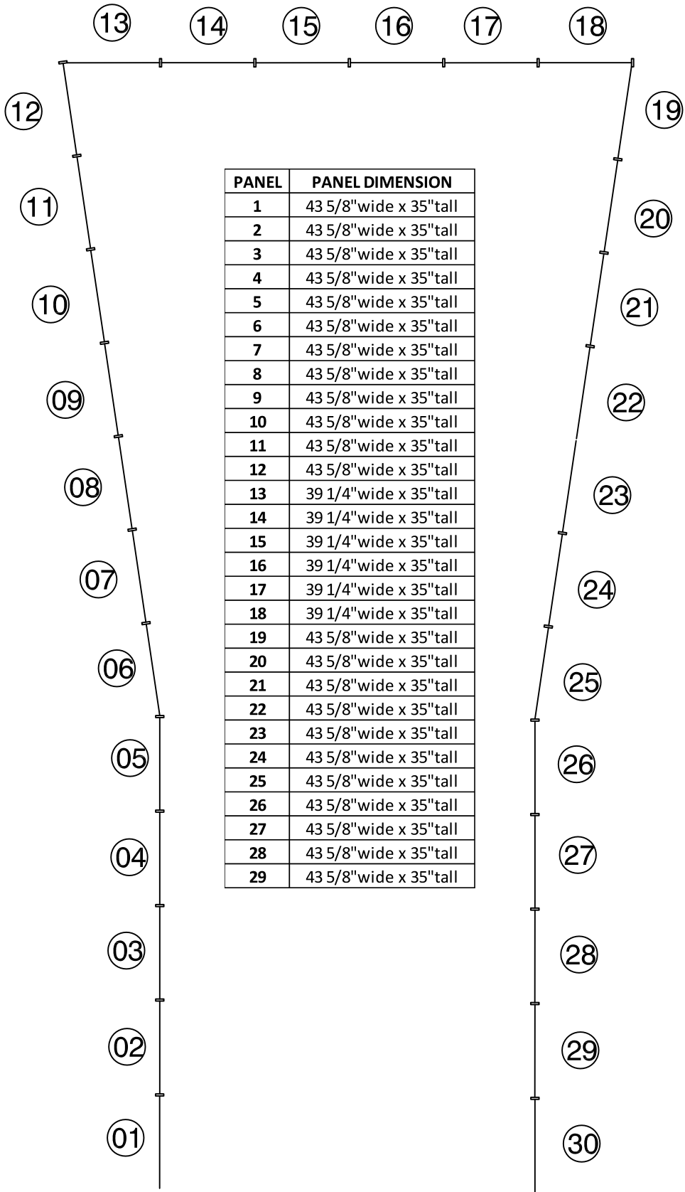
INDIVIDUAL GLASS PANELS
