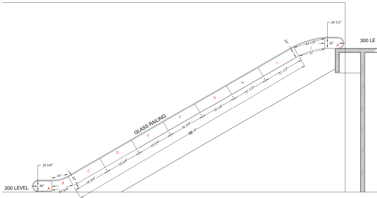
200-300 BY HALL B - SECTION
